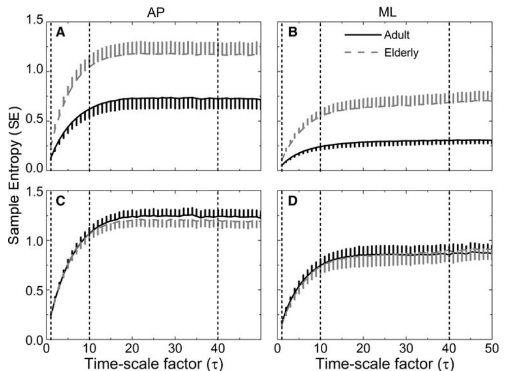
Fig. 4 a, b MSE curves (mean and SD) for postural sway time series of 14 adult and 14 older participants in the AP direction (left column) and ML direction (right column) for the regular analysis with r = 0.20 ; c, d similar plots for the COP time series after the r parameter was not adjusted
